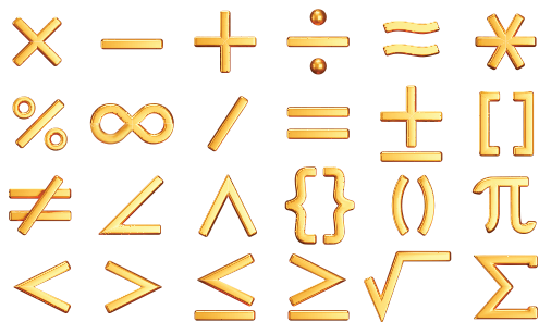
Math symbols.
